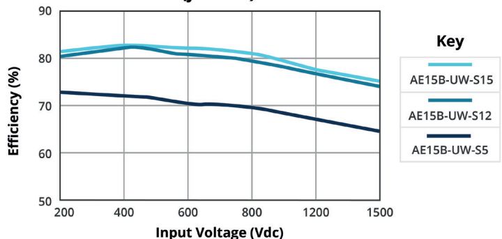
EFFICIENCY VS INPUT VOLTAGE (full load)
