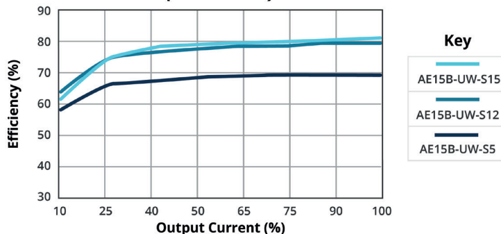
EFFICIENCY VS OUTPUT LOAD (Vin = 800 Vdc)
