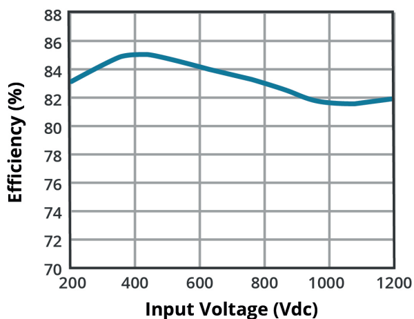
EFFICIENCY VS INPUT VOLTAGE AE40-EW-S15-DIN
